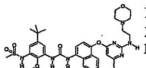
N-[5-tert-Butyl-2-methoxy-3-(3-{4-[6-methyl-2-(2-morpholin-4-yl-ethylamino)-pyrimidin-4-yloxy]-naphthalen-1-yl}-ureido)-phenyl]-methanesulfonamide;
